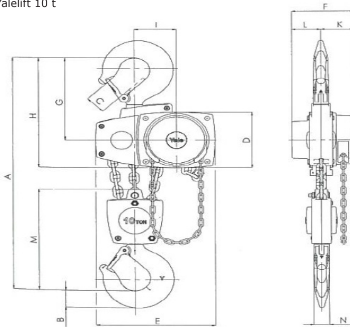
Yalelift 10 t
