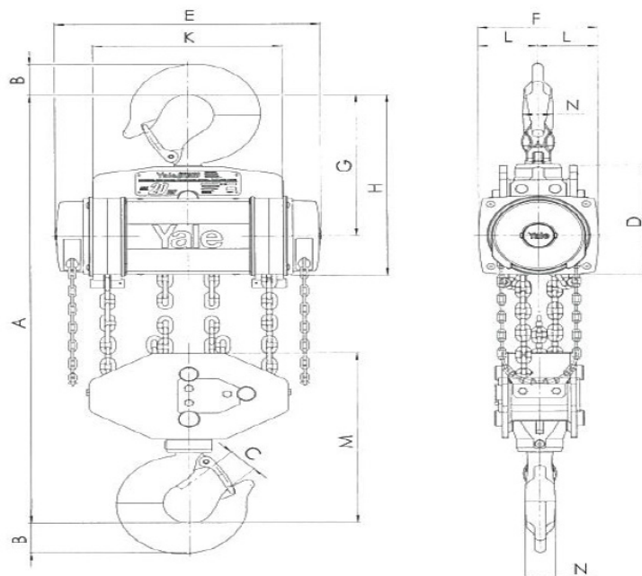
Yalelift 20 t
