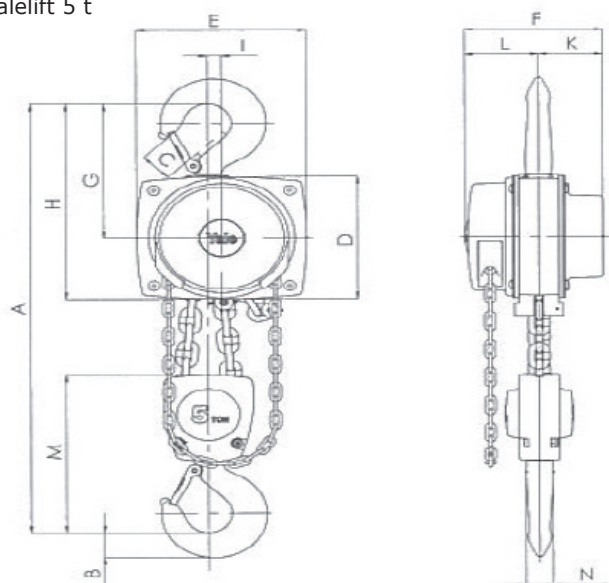
Yalelift 5 t
